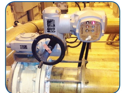
AWWA Butterfly Valve
